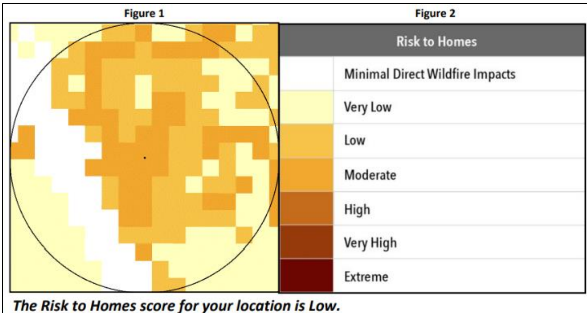
Figure 11. Part of a sample report that details Wildfire Risk. The map centers at the selected location, while the chart displays the map's legend. The colors represent the seven categories of the Conditional Risk to Potential Structures layer.
